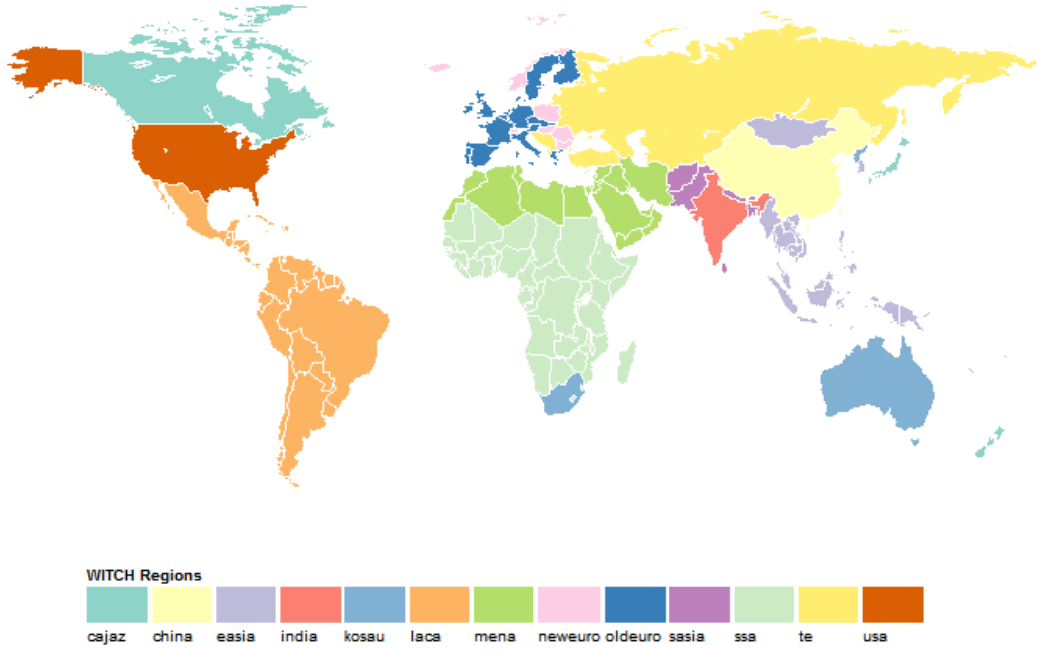
Figure 2.1: WITCH original regions
