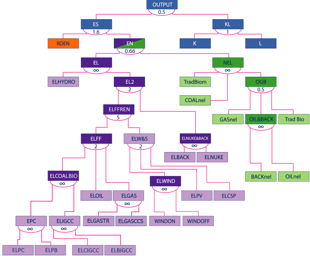
Figure 4.1: CES Production Function of WITCH
