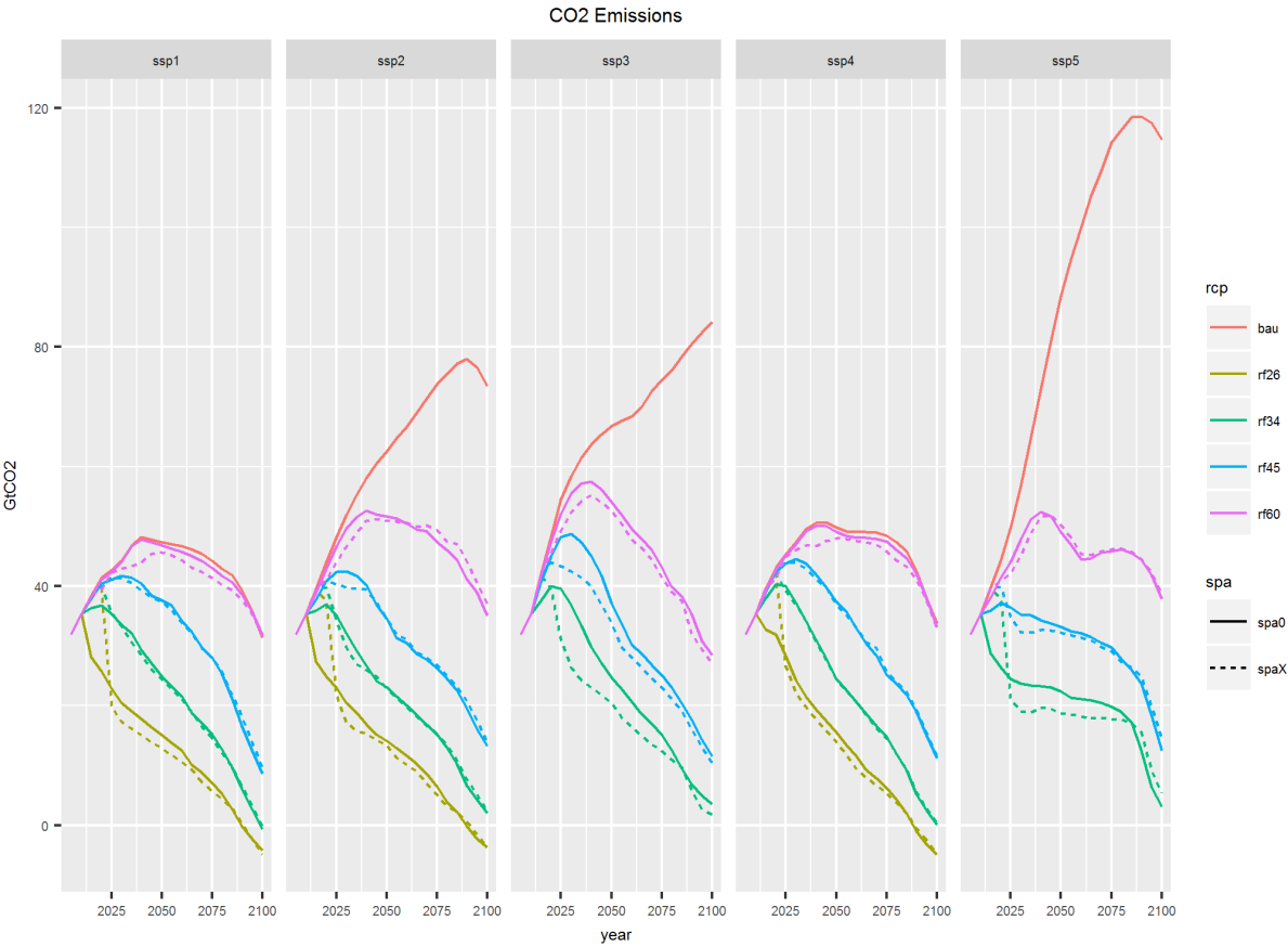
Figure 10.6: CO2 Emissions
