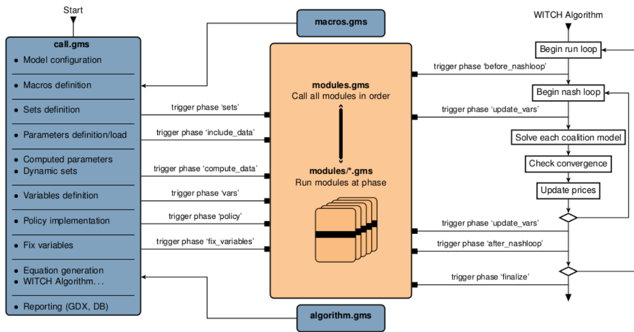
Figure 11.1: WITCH flowchart
