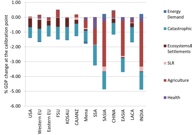
Figure 8.1: Climate change impacts at calibration point when global average temperature increases 2.5 degree Celsius above pre-industrial levels.
